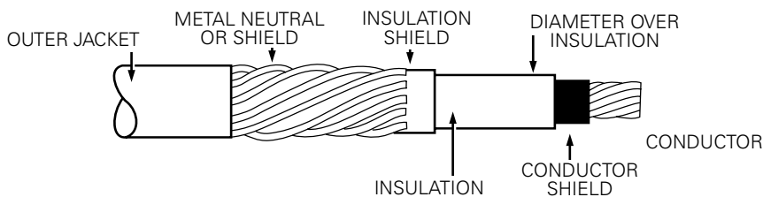
Figure 7. Cable illustration showing conductor and insulation layers.
